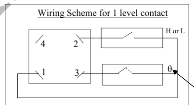
1 Level Contact
