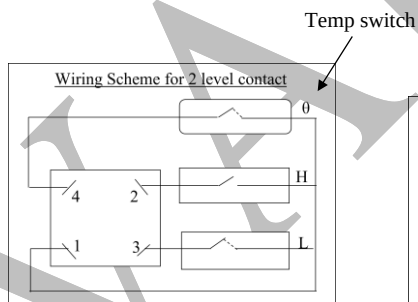
2 Level Contact
